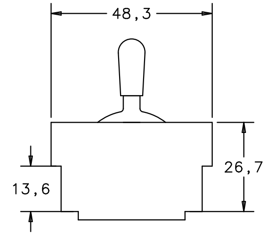
Standard 5-Wege standard 5-ways
