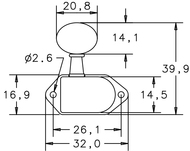
linke Mechanik left machine head
